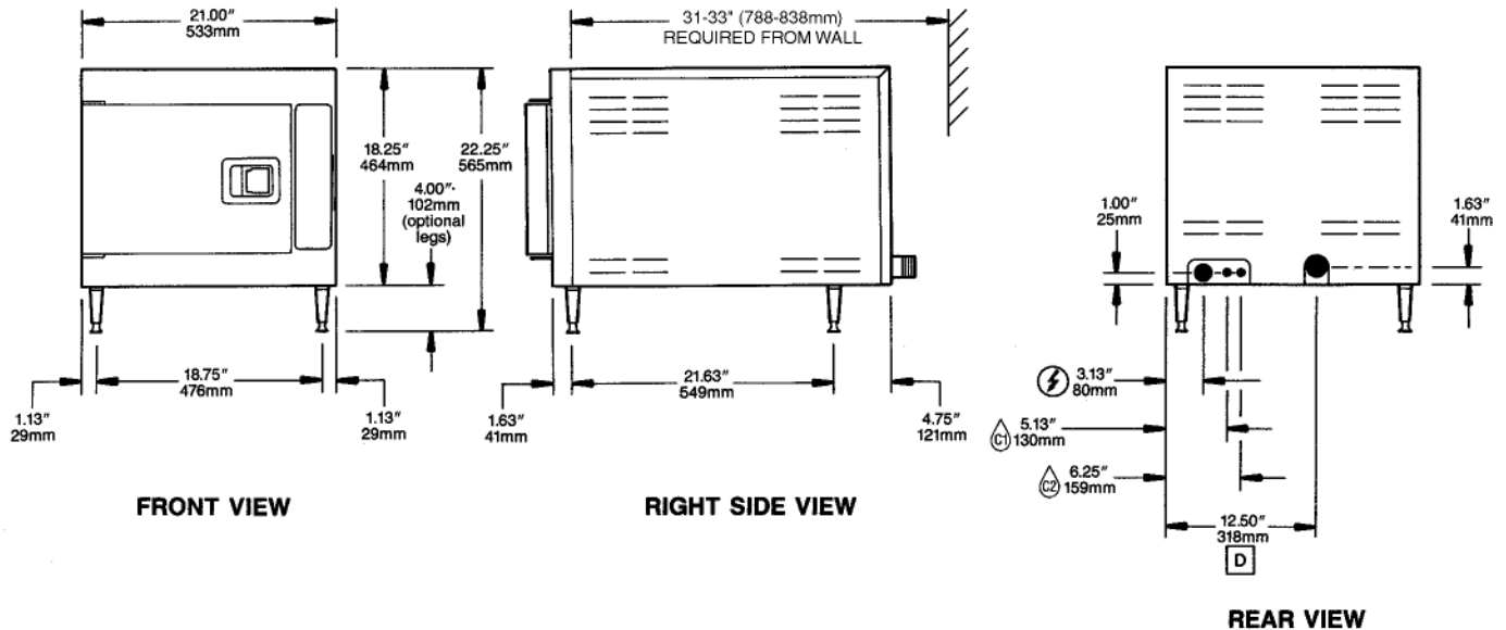
REAR VIEW
