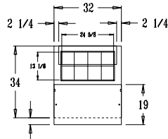
SW32-8C TOP VIEW
