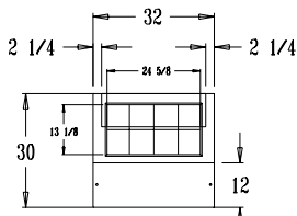
SW32-8 TOP VIEW
