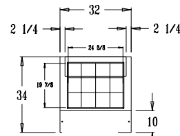
SW32-12M TOP VIEW
